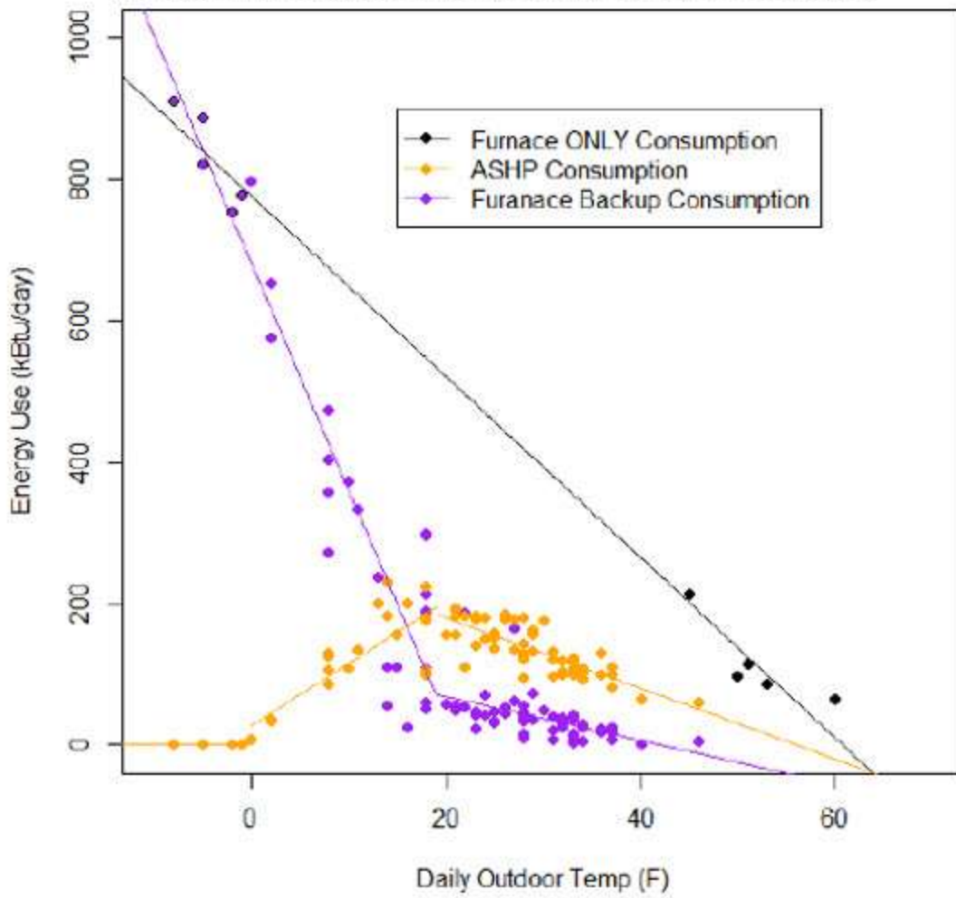
Energy use versus outdoor air temperature method from ASHP Site 2
